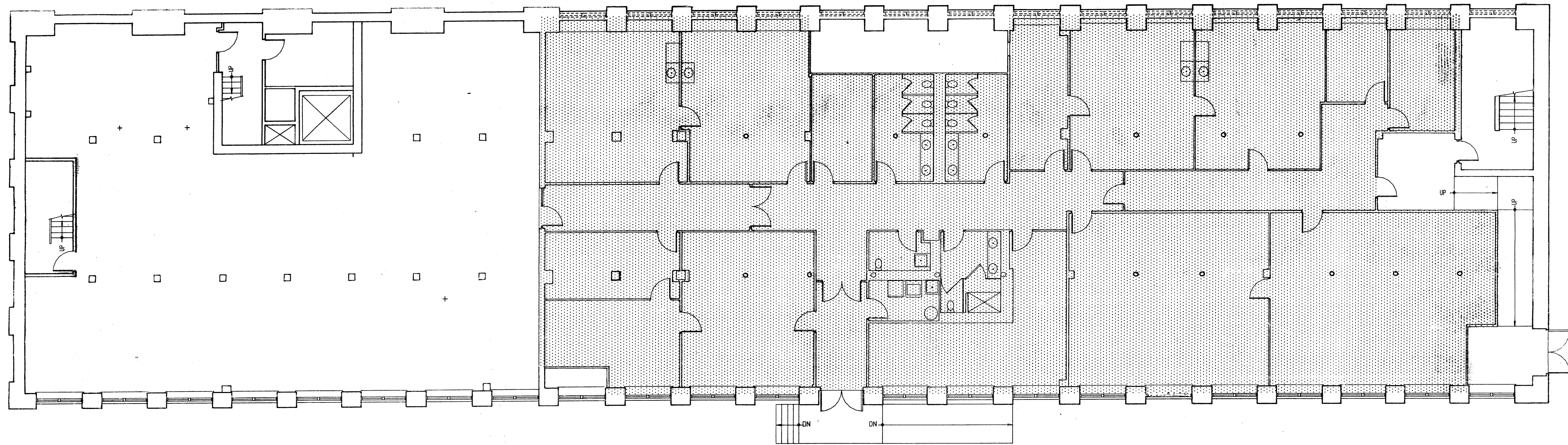
1 BASEMENT PLAN SCALE: 1/8" = 1'-0"
